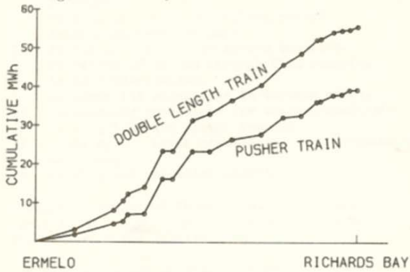
Fig. 3 Energy Consumption
